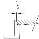
FRAME AND COVER SEATING
